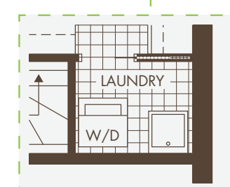
OPT. LAUNDRY LAYOUT
